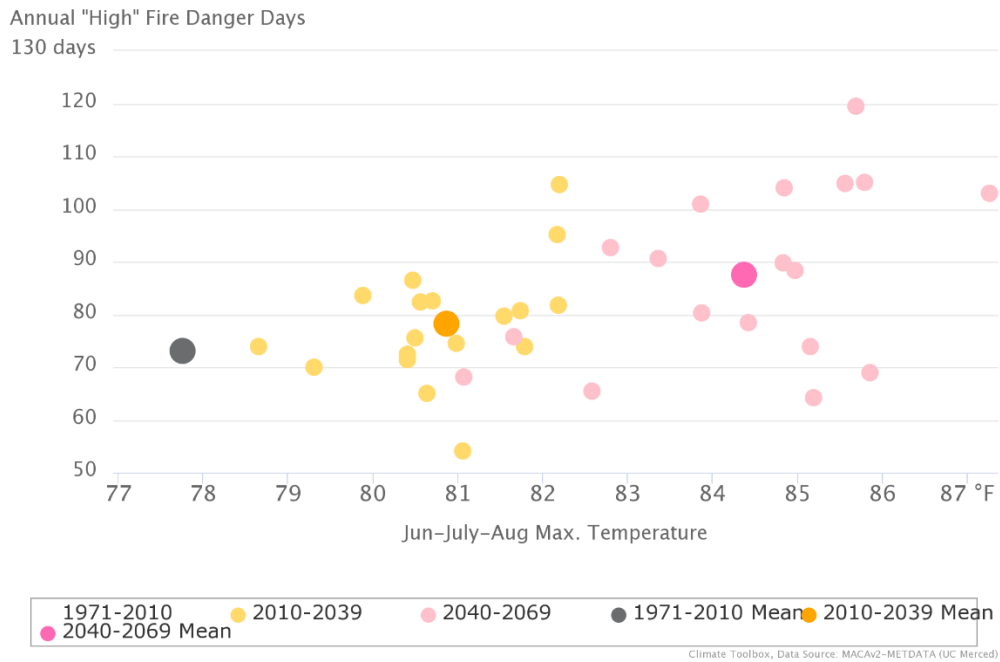
Figure 9.a.16. Potential future weather conditions in GVFPD modelled with the Climate Toolbox Future Climate Scatter (Hegewisch et al. 2021). The top graph is modelled under the RCP 4.5 scenario, where greenhouse gas emissions stabilize before the year 2100, peaking around 2040. The bottom graph is modelled under the RCP 8.5 scenario, where greenhouse gas emissions are not curtailed by 2100.
